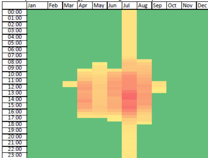
Contour plot of curtailed energy over an average 12-month period
